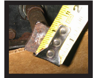
Square Nut on Drive Shaft End - 1"
