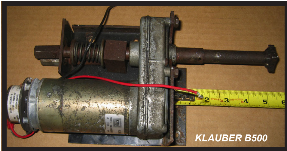
Drive shaft length - 5"
