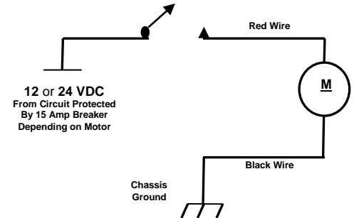
DC Motor Circuit Wiring Diagram
