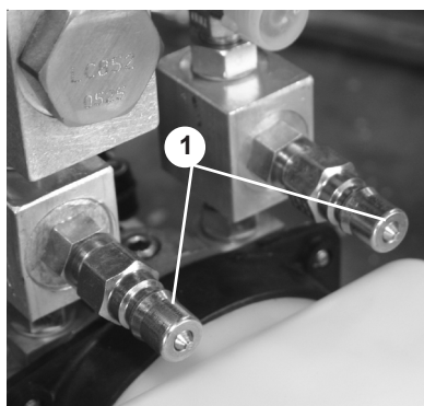
1. QUICK DISCONNECT FLUSH AND FILL FITTINGS
