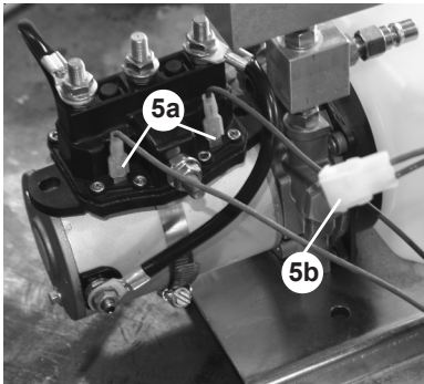
5a. WALL SWITCH LEADS- LEAD POSITIONS CAN BE SWITCHED IF SLIDEOUT MOVES OPPOSITE TO THE WAY THE WALL SWITCH READS. 5b. PLUGS IN JUST LIKE ELECTRIC MOTOR
