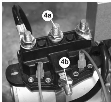
4a. POWER FROM CHASSIS BATTERY 4b. GROUND FROM CHASSIS BATTERY
