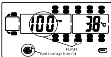
Fast Leakage Alert e.g.: 100PSI RED Light Flash
