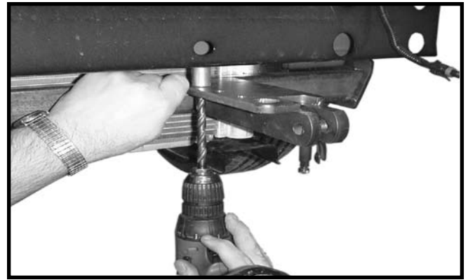
14. Drill two 3/8" holes in bumper using base plate chain anchor as a guide insert bolts and tighten (use shims if needed).
