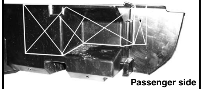
15. Notch plastic filler panel where it is marked around base plate on each side and replace.
