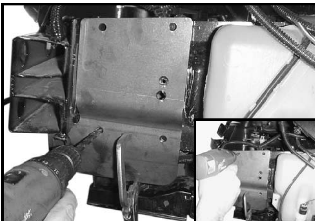
13. Drill bottom two 3/8" holes (on each side) insert bolts and tighten, drill top two 3/8" holes (on each side) place spacer bushings on each as shown on front cover with the longer spacers on the drivers side and the shorter spacers on the passenger side. NOTE: Use Blue LOCTITE ® on threads and tighten bolts according to bolt chart on front page.
