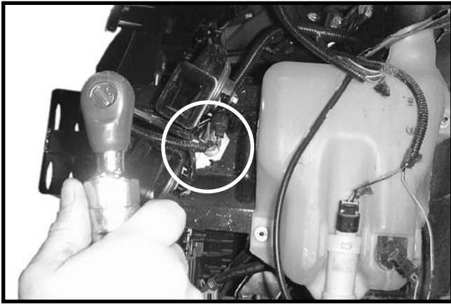
11. Remove one bolt from horn. Bolt will not be reused.
