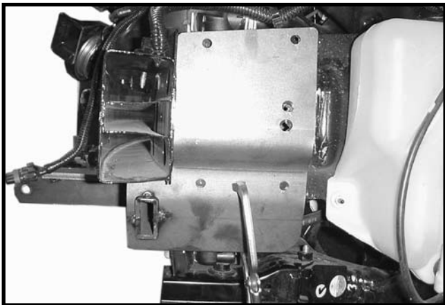
12. With an assistant, slide base plate up onto frame and forward to bumper make sure horn bolt hole and air box holes line up, then clamp.
