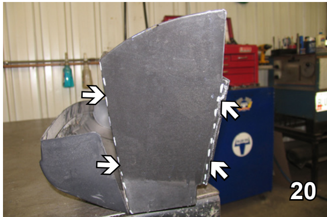
20. Using a utility knife, cut the ends off of the plastic air dam from below the bumper.
