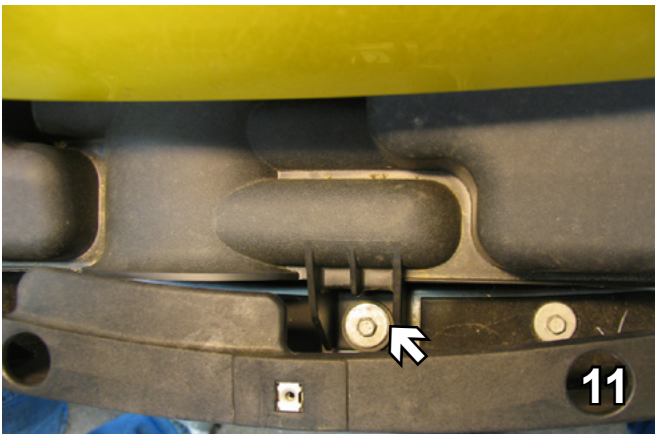
11. Up on top, remove one bolt using a 10MM socket. Set aside bolt for later reinstallation.
