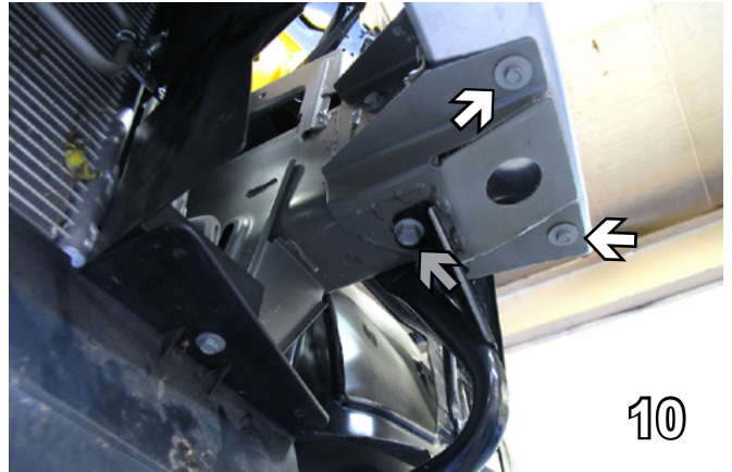
10. Remove three bolts underneath the bumper. Use a 10MM socket on the top two and a 15MM socket for the bottom one (grey arrow). Set aside bolts for later reinstallation.
