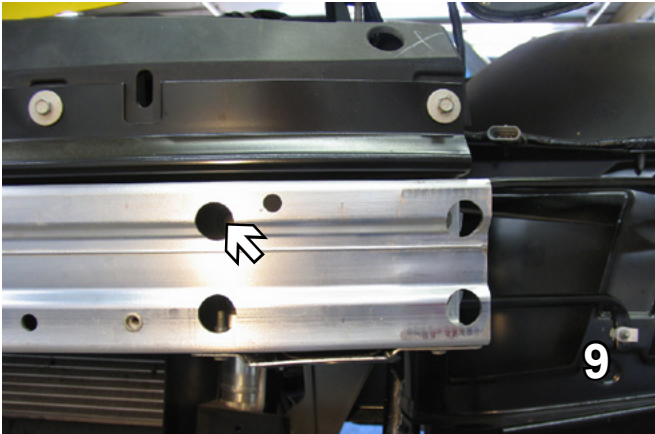
9. Using a 13MM socket, remove two more bolts from both sides. Set bolts aside to be reinstalled later.
