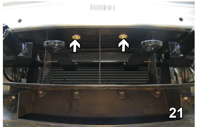
21. Reinstall bumper and air baffle over the top of the base plate. Attach with two center bolts.
