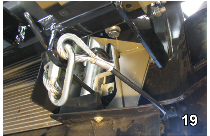
19. Attach the permanent baseplate safety cables to the provided convenience link on the baseplate. The photo above shows the recommended installation of the cables to frame of vehicle. Additional options may interfere with suggested mounting; in this case, secure the cables to a solid piece of the frame as described in the instructions included with the permanent baseplate safety cables. Be sure the safety cables do not rub against any hoses or moving parts. Do this on BOTH sides of the vehicle.
