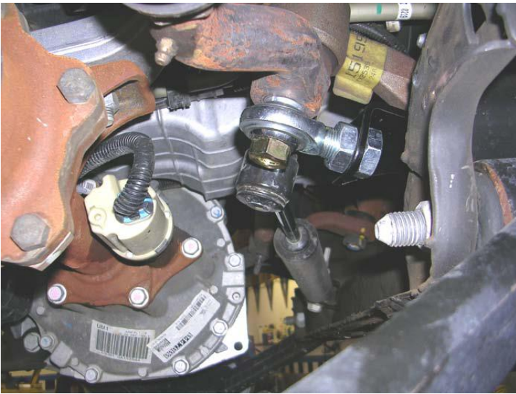
Figure 3: idler arm bracket installed
